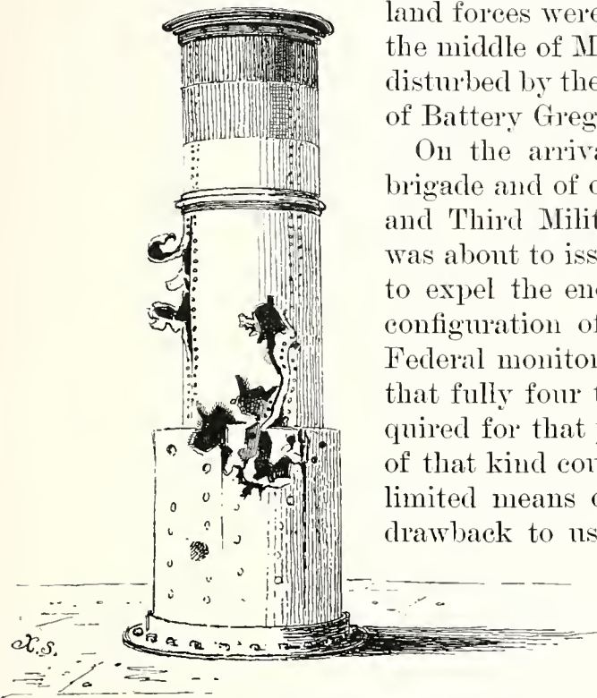
EFFECT OF THE SHOT FROM FORT SUMTER ON THE PLATING AND THE SMOKE-STACK OF THE MONITOR "WEEHAWKEN." FROM PHOTOGRAPHS.
